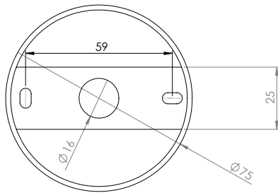
Back box 75 A
