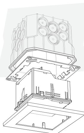
Flush-mounted installation (set into concrete ceiling)
