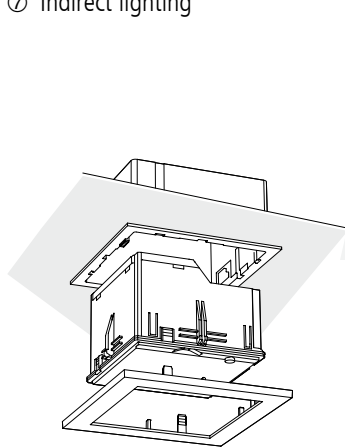
False ceiling installation (false ceilings)
