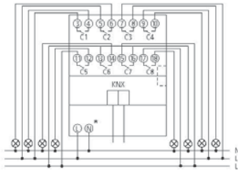
RMG 8 S KNX or RME 8 S KNX (*only with RMG 8 S KNX)
