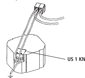
Fig. 1: Mounting US 1 KNX directly on the bus coupler
